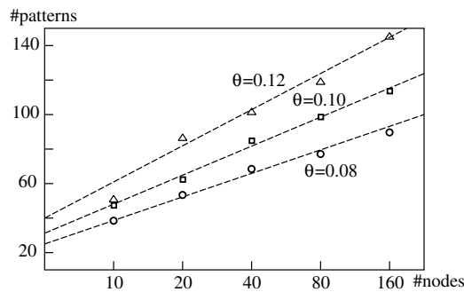
Fig. 2. Result on the number of expression patterns required to identify the noisy Boolean network of K = 2 correctly. Note that the X-axis is log scaled.
