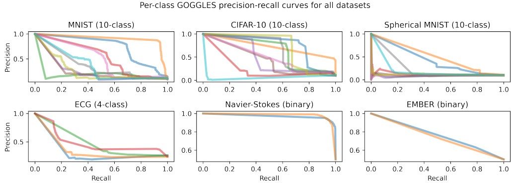
Figure 6: Class-wise precision recall curves using GOGGLES across datasets. Despite having 100% coverage on all tasks, GOGGLES has wildly varying per-class performance that becomes more pronounced as the number of classes increases. Permuted MNIST is not shown as the predictions are the same as on MNIST due to the permutation invariance of PCA.
