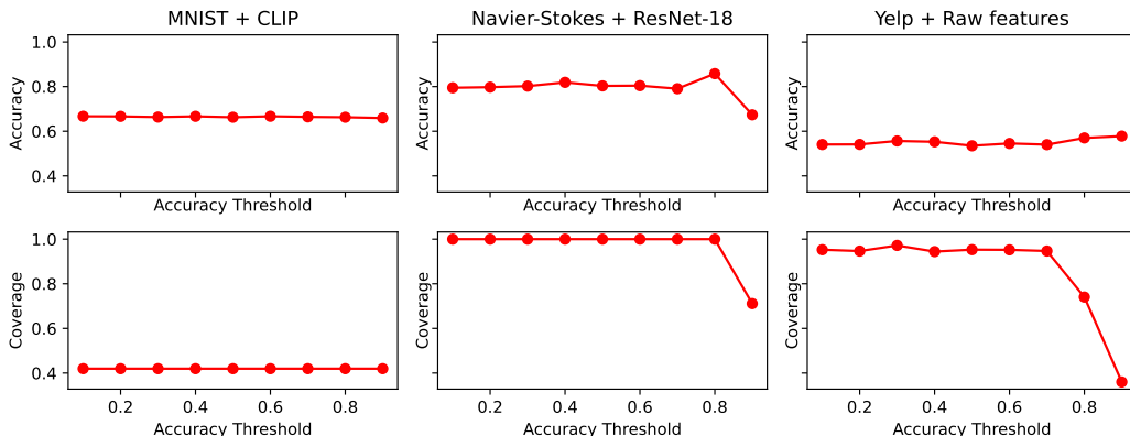
Figure 7: Tuning the threshold parameter of the automated version of IWS does not lead to significant improvements in performance, and can hurt coverage if it is set to be too high.
