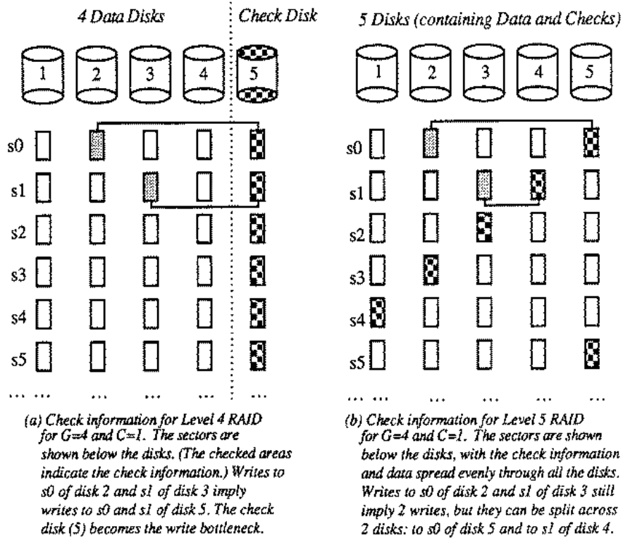
Figure 4. Location of check information per sector for Level 4 RAID vs. Level 5 RAID.
