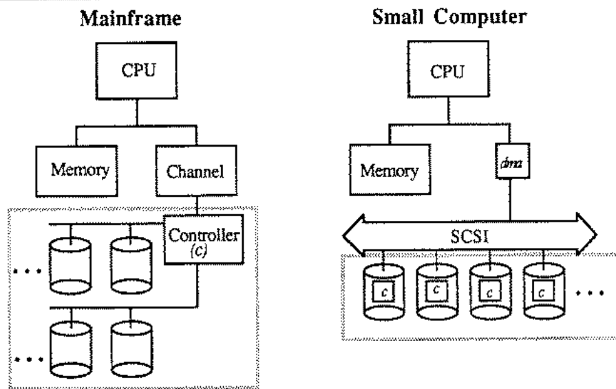
Figure 1. Comparison of organizations for typical mainframe and small computer disk interfaces. Single chip SCSI interfaces such as the Adaptec AIC-500 allow the small computer to use a single chip to be the DMA interface as well as provide an embedded controller for each disk. (The price per megabyte shown in Table I includes everything in the dotted boxes.)
