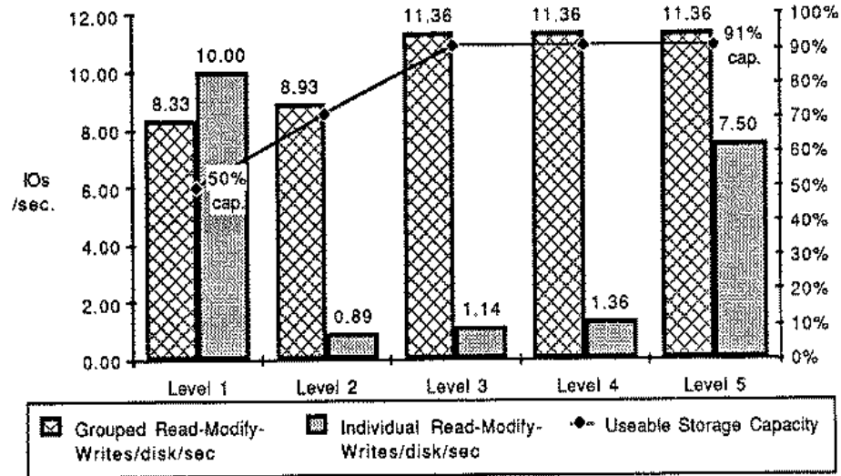
Figure 5. Plot of Large (Grouped) and Small (Individual) Read-Modify-Writes per second per disk and useable storage capacity for all five levels of RAID ( D=100 , G=10 , I/O=30/sec , S=1.2 ). To scale performance to other speed disks, simply multiply these numbers by the ratio to 30 I/O's/sec.
