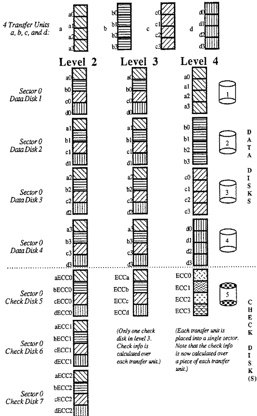
Figure 3. Comparison of location of data and check information in sectors for RAID levels 2, 3, and 4 for G=4 . Not shown is the small amount of check information per sector added by the disk controller to detect and correct soft errors within a sector.
