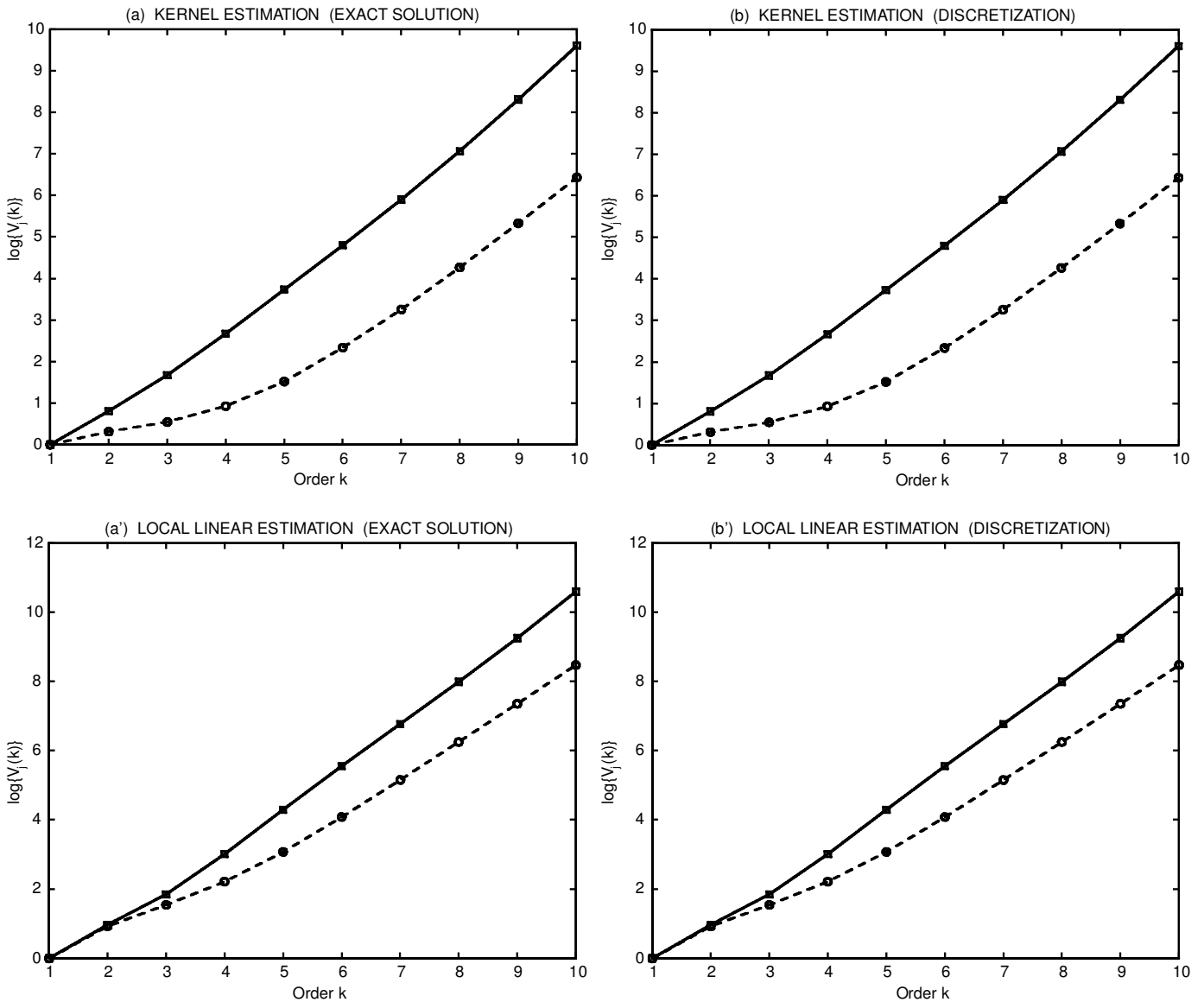
Figure 3. Simulated Values of \log\{V_j(k)\} Versus Order k for Geometric Brownian Motion dX_t = (.087 + .178^2/2)X_t dt + .178X_t dW_t . The index j = 1 (-o-) refers to the drift estimator \hat{\mu}_{1,\Delta}(1.0) ; j = 2 (-□-) refers to the squared diffusion estimator \hat{\mu}_{2,\Delta}(1.0) . Plots (a) and (a') are based on the same sets of sample paths generated from the exact solution X_t = X_0 \exp\{.087t + .178W_t\} , whereas plots (b) and (b') are based on the same sets of sample paths generated by the discretization scheme (34).
