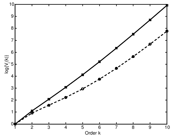
Figure 1. Theoretical Values of \log\{V_j(k)\} Versus Order k . The factors V_j(k) are given in Theorem 2, where j = 1 (---) refers to drift \mu(\cdot) and j = 2 (—□) refers to squared diffusion \sigma^2(\cdot) .
