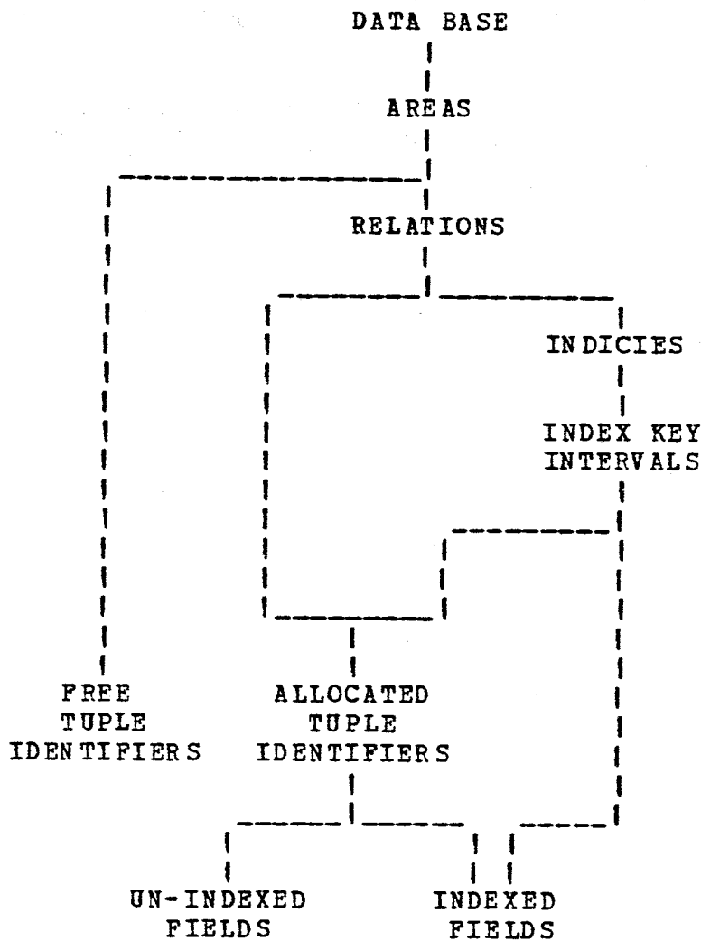
Figure 5. A lock graph.
