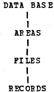
Figure 1. A sample lock hierarchy.
