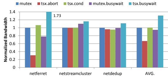
Figure 6: Intel TSX performance on user-level TCP/IP stack. Reports server-side read bandwidth.
