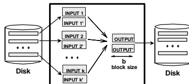
B main memory buffers, k-way merge
