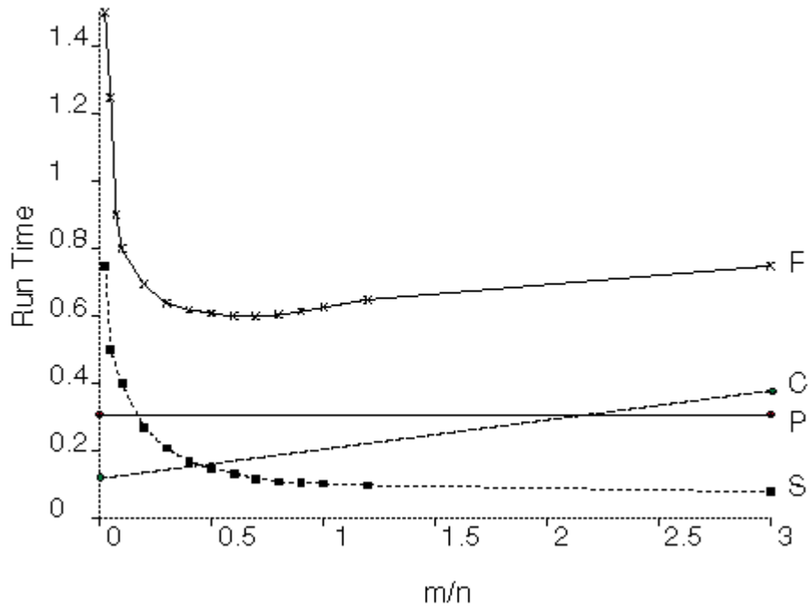
Figure 1: The time contribution of the various procedures to the total run time as a function of m/n. P=permutation time, C=classification time, S=straight-insertion time, F=total time for Flashsort1.
