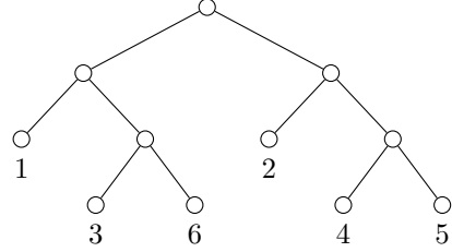
Figure 11: Tree insensitive to non-sibling transposition
