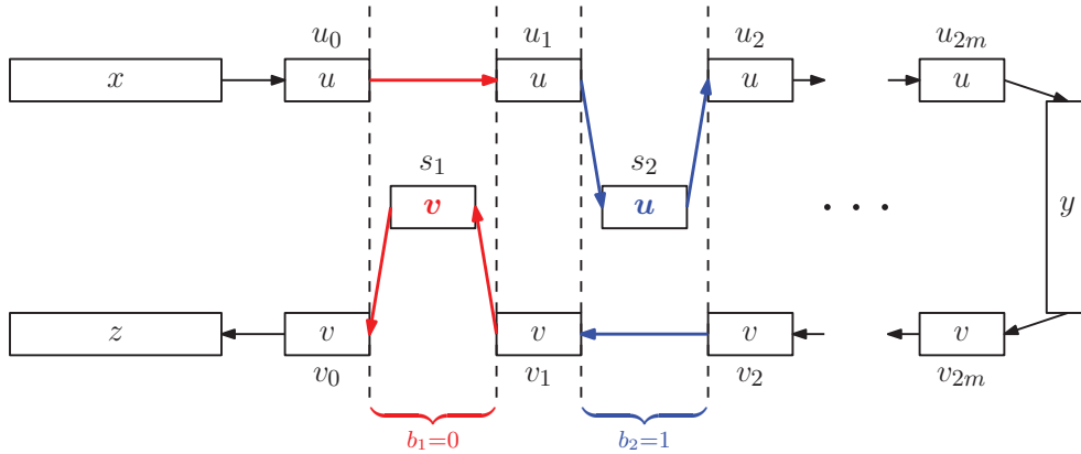
FIG. 6.1. Constructing the string w_b from b . (Note that the strings v and z are drawn right to left.)
