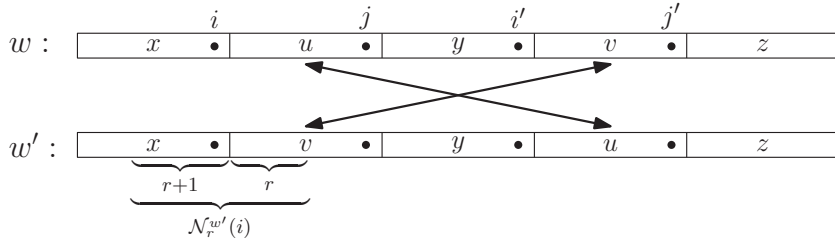
FIG. 5.1. r -swapping w = xuyvz to w' = xvyuz .
