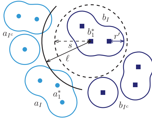
FIG. 4.8. Diagram for Case 4.
