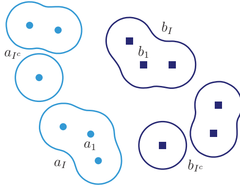
FIG. 4.6. Diagram for Case 4 when b_1 is close to some component of \bar{b} .
