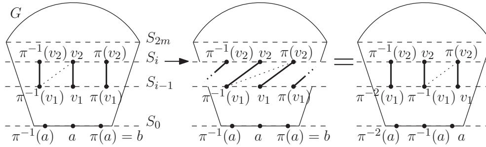
FIG. 4.3. Diagram for rotating the shell of radius i around S_0 when w_i = 1 .
