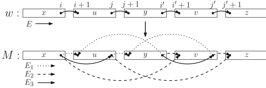
FIG. 5.3. Constructing the structure M from the string w .
