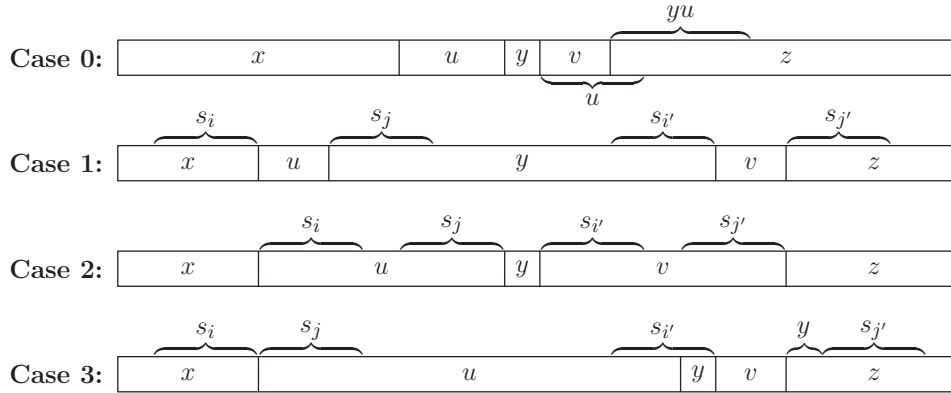
FIG. 5.4. The cases in the proof of Lemma 5.4.
