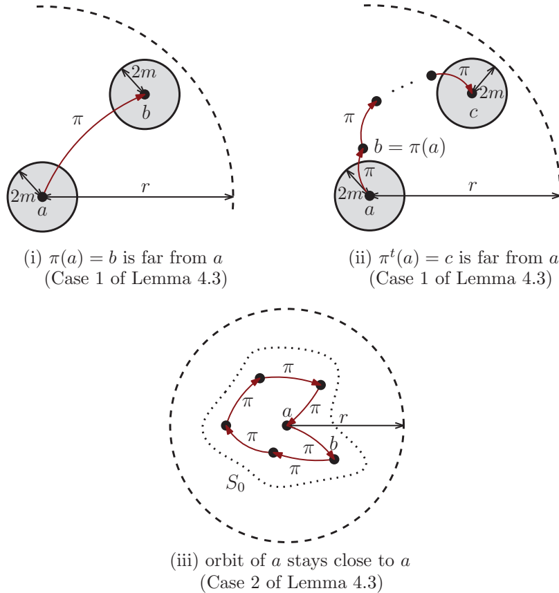
FIG. 4.2. Diagram for the general unary case. ( r is the radius of the domain of \pi .)
