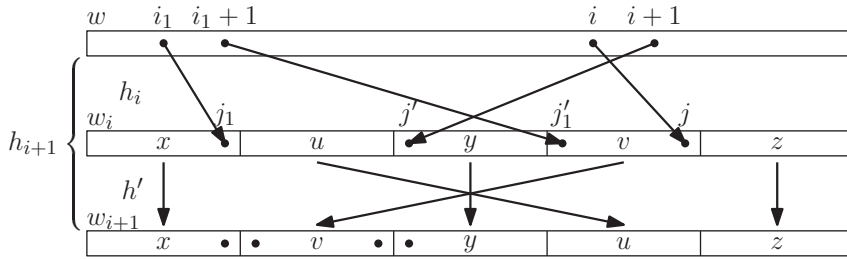
FIG. 5.2. Constructing h_{i+1} from h_i and w_i .
