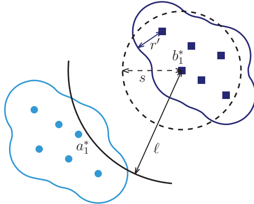
FIG. 4.7. Diagram for Case 3.
