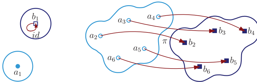
FIG. 4.5. Diagram for the hybrid isomorphism from Case 4 that maps \bar{h} = (b_1, a_2, \dots, a_k) to \bar{b} = (b_1, b_2, \dots, b_k) .
