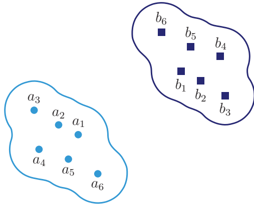
FIG. 4.4. Diagram for Case 3.
