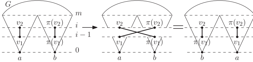
FIG. 4.1. Diagram for swapping the neighborhoods of a and b of radius i , conditioned on w_i = 1 .
