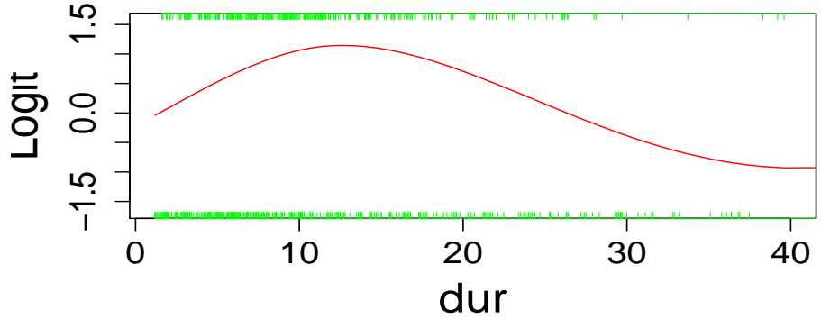
Figure 9: Estimated logit component for dur .
