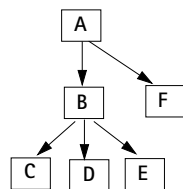
Dominator Tree
