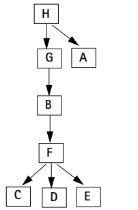
Postominator Tree
