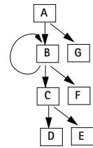
Control Dependence Graph
