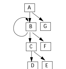
Control Dependence Graph
