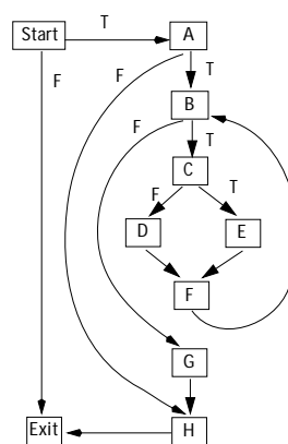
Control Flow Graph
