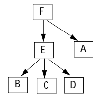
Postominator Tree
