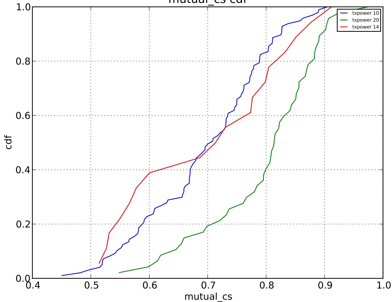
mutual_cs cdf
