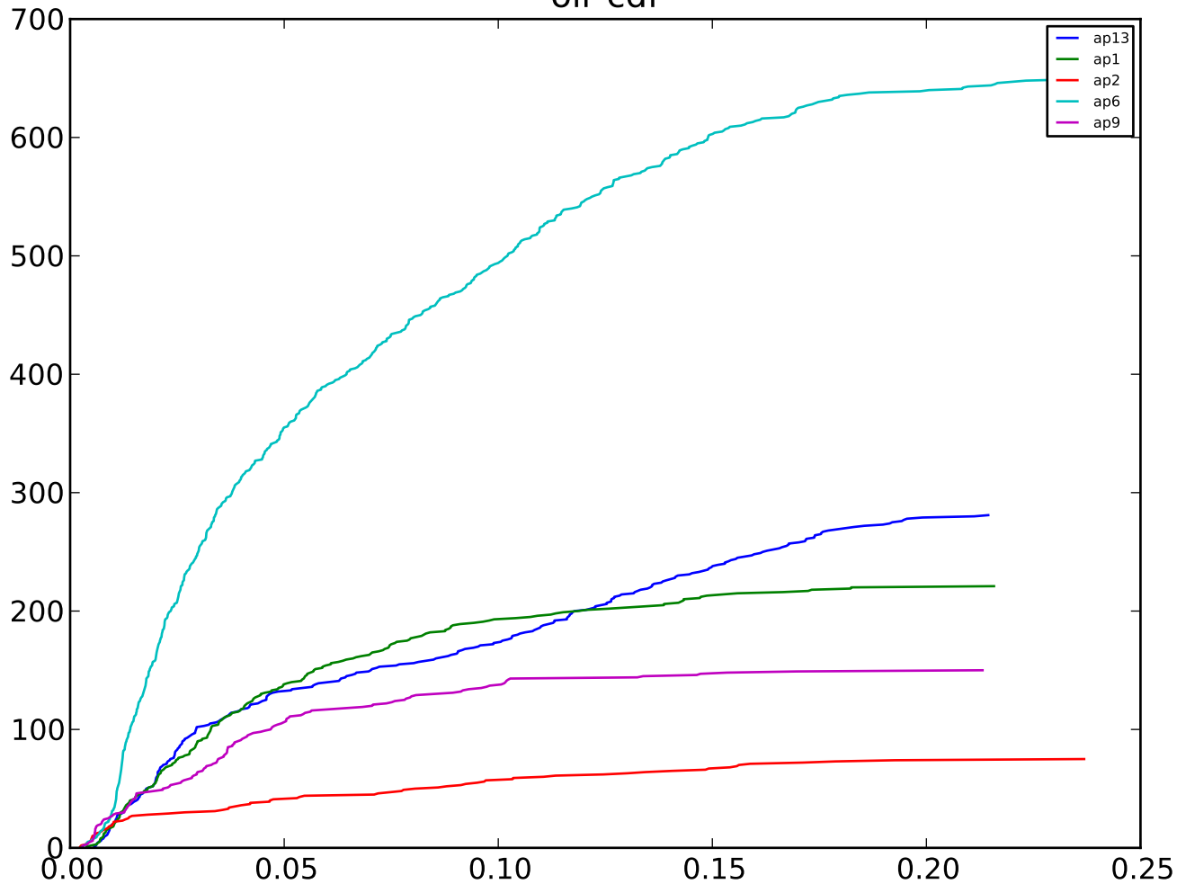
olr cdf
