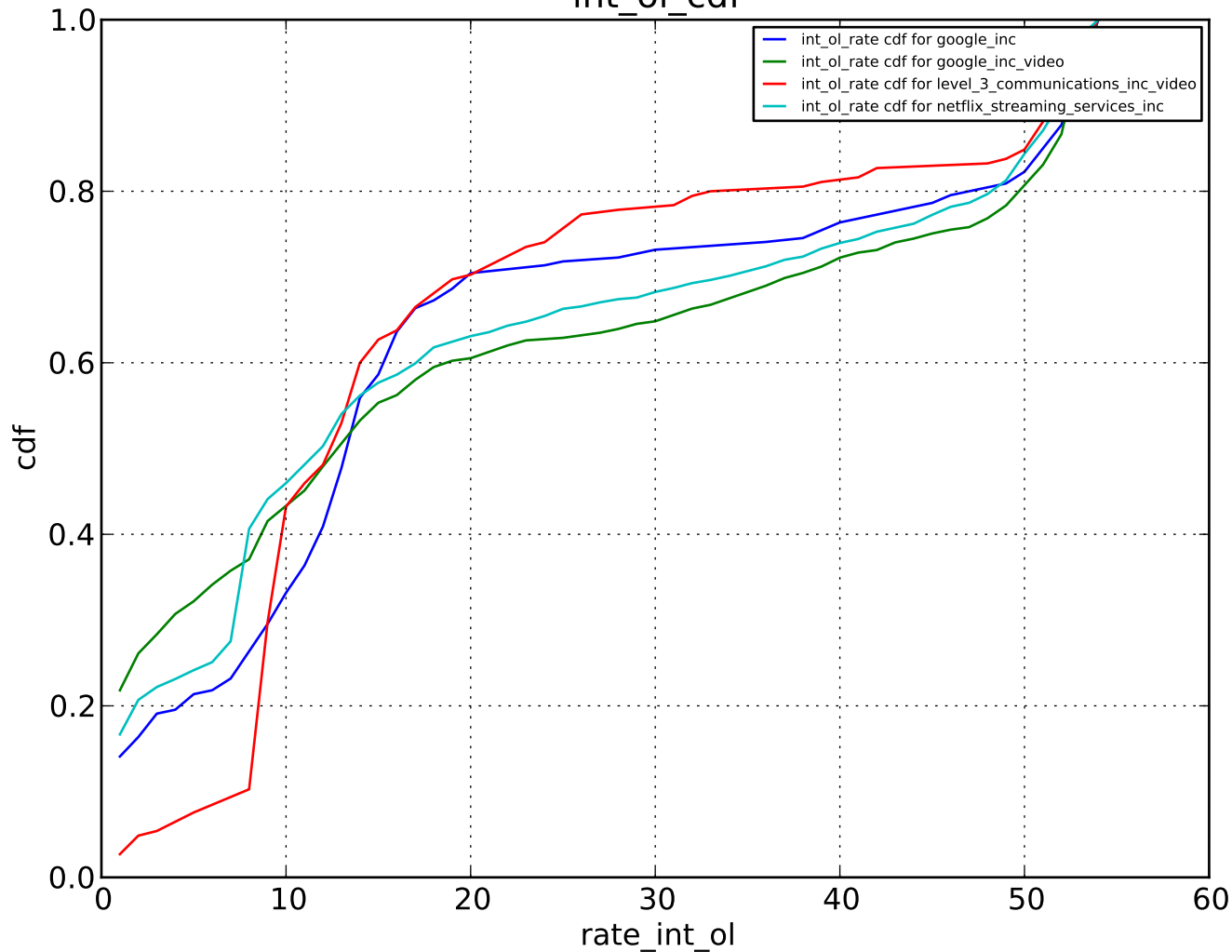
int_ol_cdf
