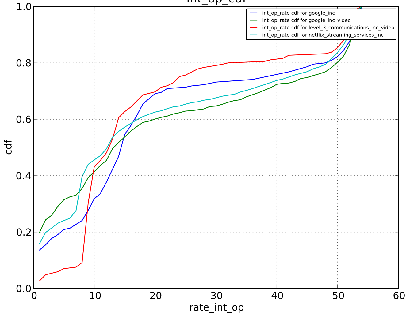
int_op_cdf
