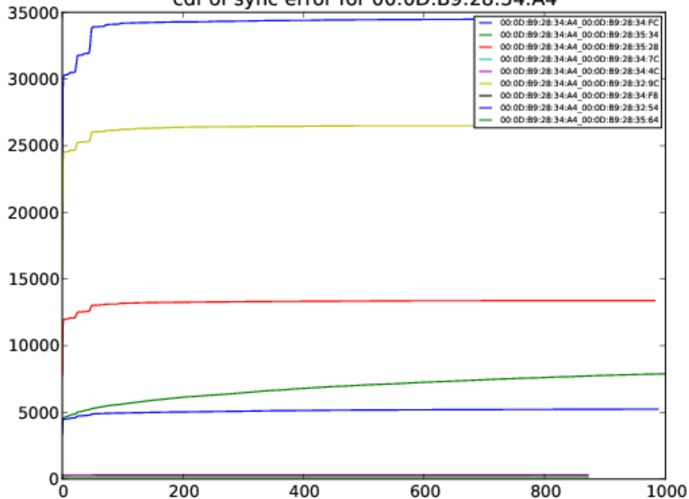
cdf of sync error for 00:0D:B9:28:34:A4
