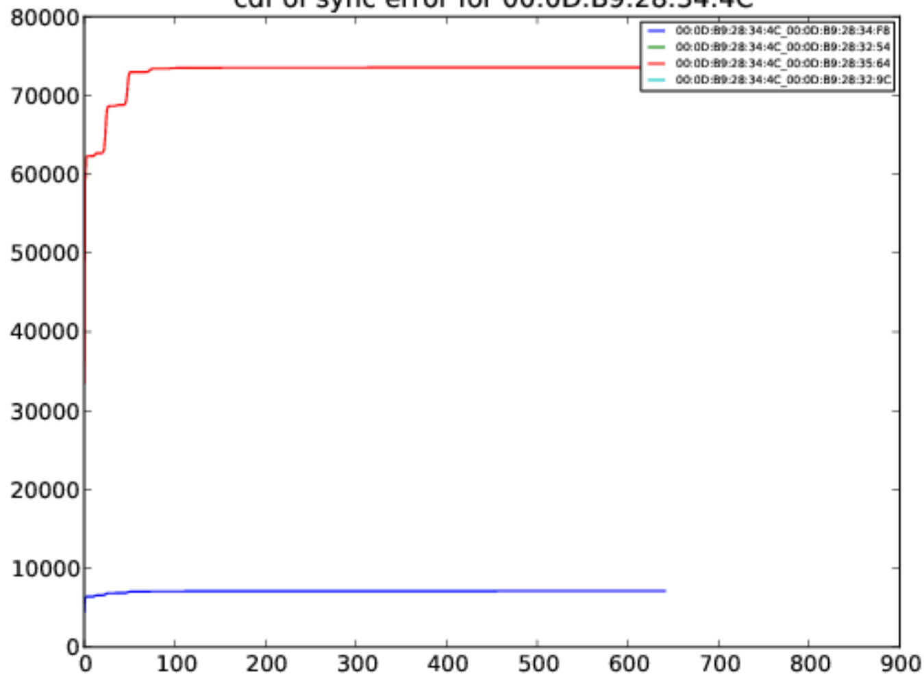
cdf of sync error for 00:0D:B9:28:34:4C
