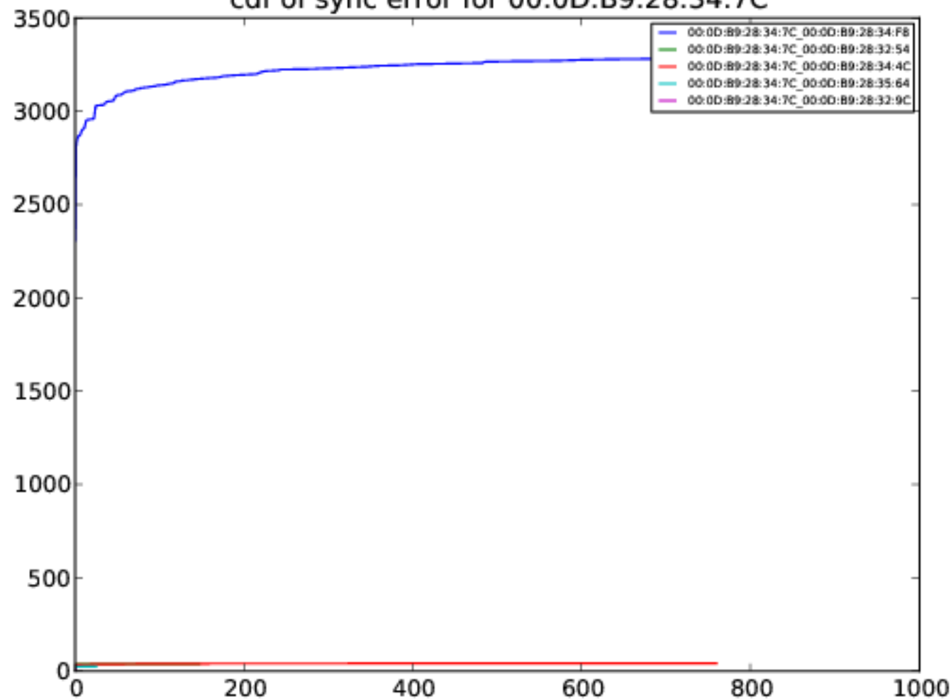
cdf of sync error for 00:0D:B9:28:34:7C
