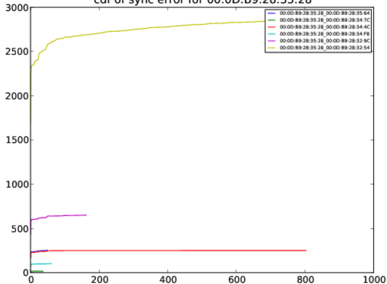
cdf of sync error for 00:0D:B9:28:35:28
