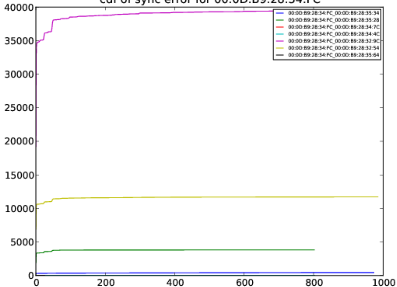
cdf of sync error for 00:0D:B9:28:34:FC
