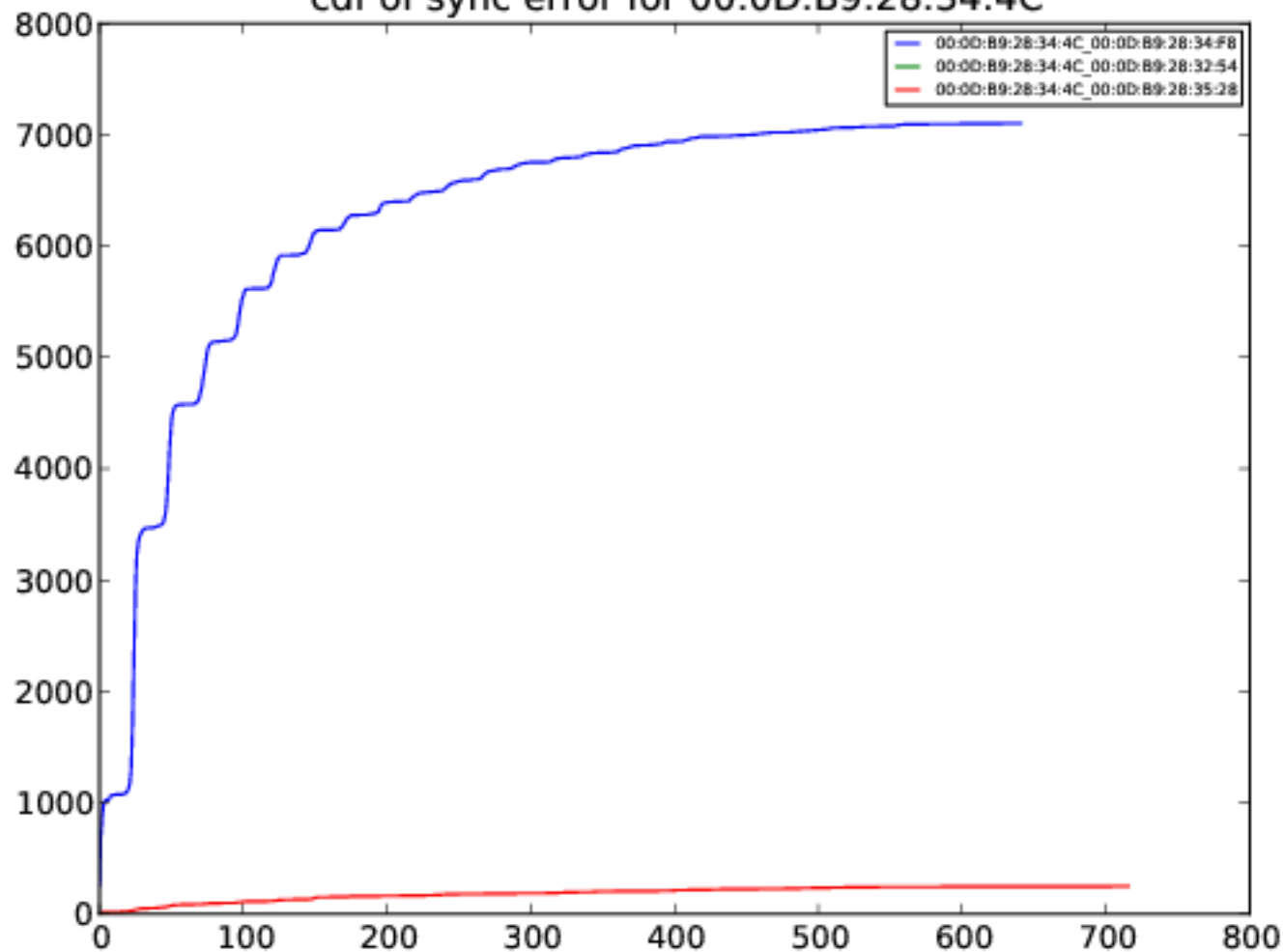
cdf of sync error for 00:0D:B9:28:34:4C
