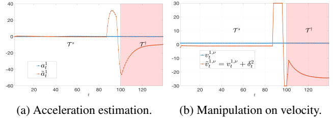
Figure 8: Acceleration reduces significantly as the velocity measurement drops after step 96. This in turn causes the KF velocity estimation to decrease fast.
