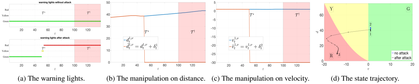
Figure 10: Greedy attack on the MIO+1 dataset.
