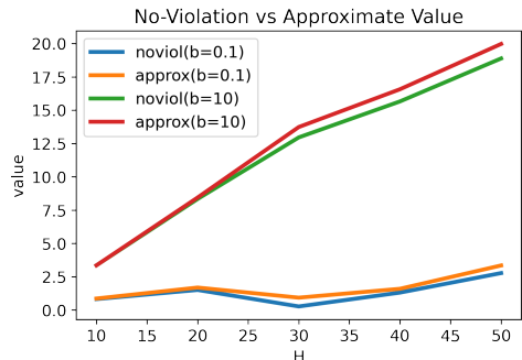
Figure 1: Value comparison of our relative approximation and feasibility scheme.
