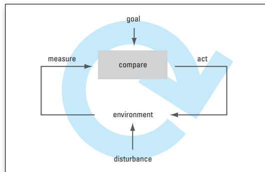
► Self-regulating system
