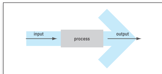
► Linear system
