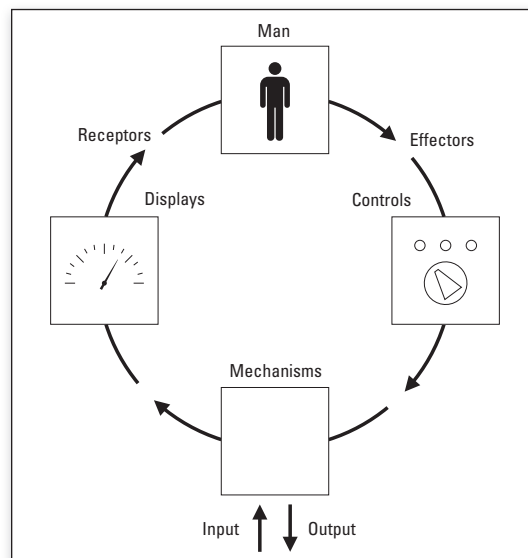
► Man-Machine system
