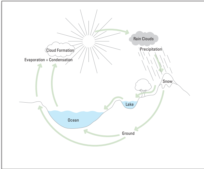
► Water cycle
