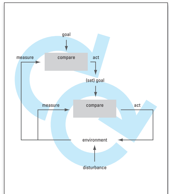
► Learning system
