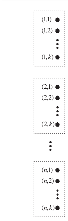
Figure 1: Generator Matchgate \Gamma . We omit all the internal structures. All the kn external nodes are labeled by a pair of integers and they are all on the outer face.
