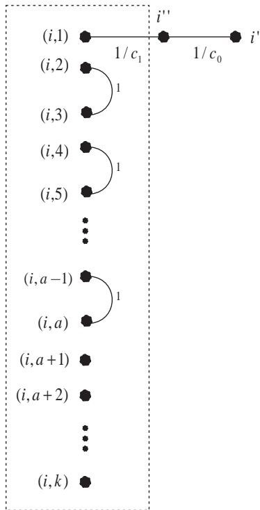
Figure 3: Modify the i -th block of \Gamma to get the i -th external node of \widehat{\Gamma}
