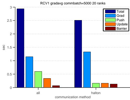
Figure 8. This figure shows the time consumed by different steps in distributed SVM for RCV1 workload for synchronous training.
