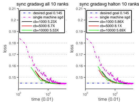
Figure 10. This figure shows convergence (loss vs time in seconds) for RCV1 dataset for MALT-all (left) and MALT-halton(right) for different communication batch sizes. We find that MALT halton converges faster than MALT all .
