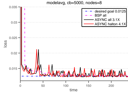
Figure 11. This figure shows convergence (loss vs time in seconds) for splice dataset for MALT-all and MALT-halton. We find that MALT halton converges faster than MALT all .
