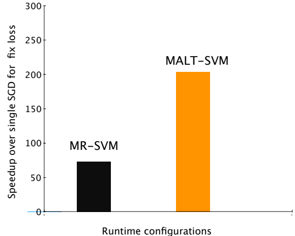
Figure 5. This figure shows convergence with PASCAL workload for MALT all-all SVM with MR-SVM. We achieve super-linear speedup for some workloads because of the averaging effect from parallel replicas [51]. We find that MALT all-all SVM is about 3X faster than map-reduce SVM implemented over infiniband.
