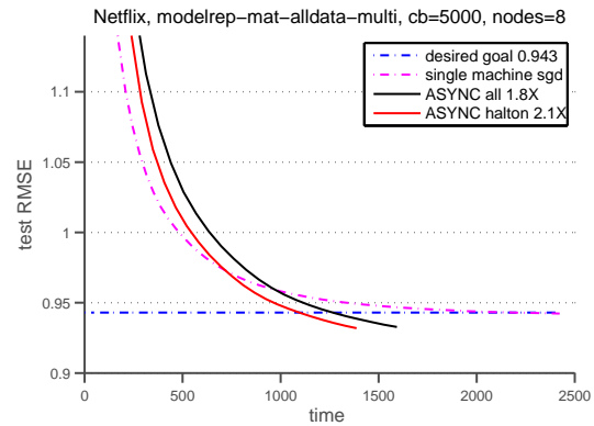
Figure 12. This figure shows the test error vs time in seconds processed for matrix factorization with the Netflix dataset. We train asynchronously over eight machines, and use grad-replace gather function.
