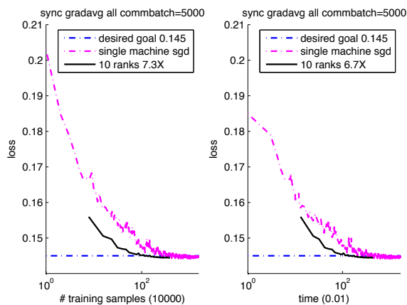
Figure 4. This figure shows convergence for RCV1 workload for MALT all-all with a single machine workload. We find that MALT all-all converges quicker to achieve the desired accuracy.
