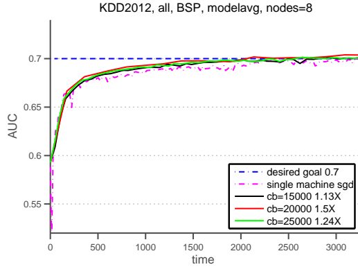
Figure 6. This figure shows the AUC (area under curve) vs time taken to speedup (in seconds) for a three layer neural network for text learning (click prediction). We find that provides speedup over a single node.
