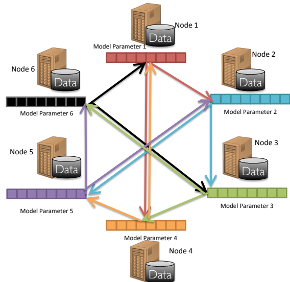
Figure 3. Halton series exchange of model updates ( N = 6 ). Each i th machine sends updates to \log(N) (2 for N = 6 ) nodes. (to N/2 + i and N/4 + i ). As number of nodes N increases, the outbound nodes follows Halton series ( N/2, N/4, 3N/4, N/8, 3N/8.. ). All arrows are uni-direction. As number of nodes(N) grow, total number of updates transmitted increases O(N \log N) .
