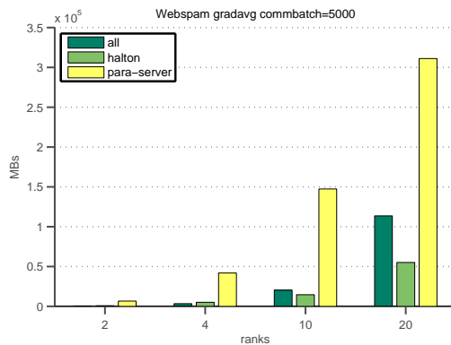
Figure 13. This figure shows the network costs for MALT all-all , MALT halton and parameter server for the whole network for webspam workload. We find that MALT halton reduces network communication costs and provides fast convergence.
