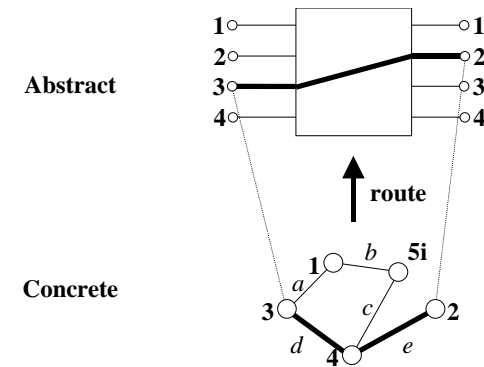
Fig. 8. Composing switches in a mesh.
