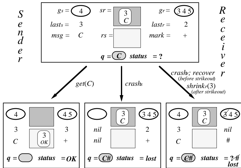
Figure 3. Some states and transitions of G
