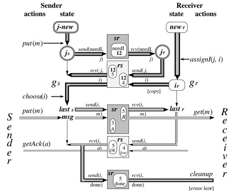
Figure 7. The flow of information in H
