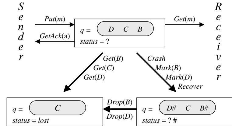
Figure 2. Some states and transitions of D
