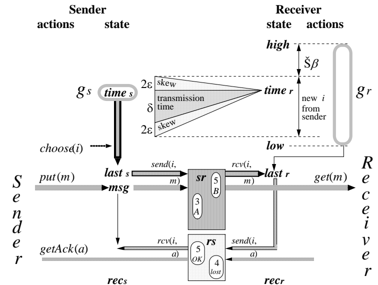
Figure 6. The flow of information in C
