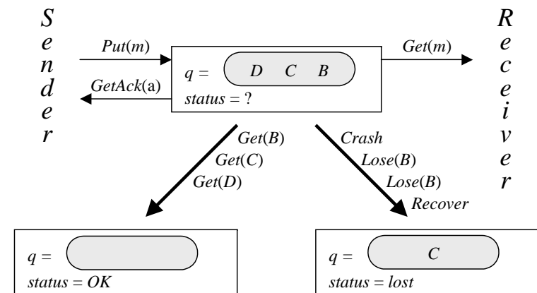
Figure 1. Some states and transitions for S
