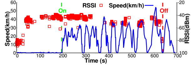
Figure 4: Identify where the passenger get on or off the bus.
