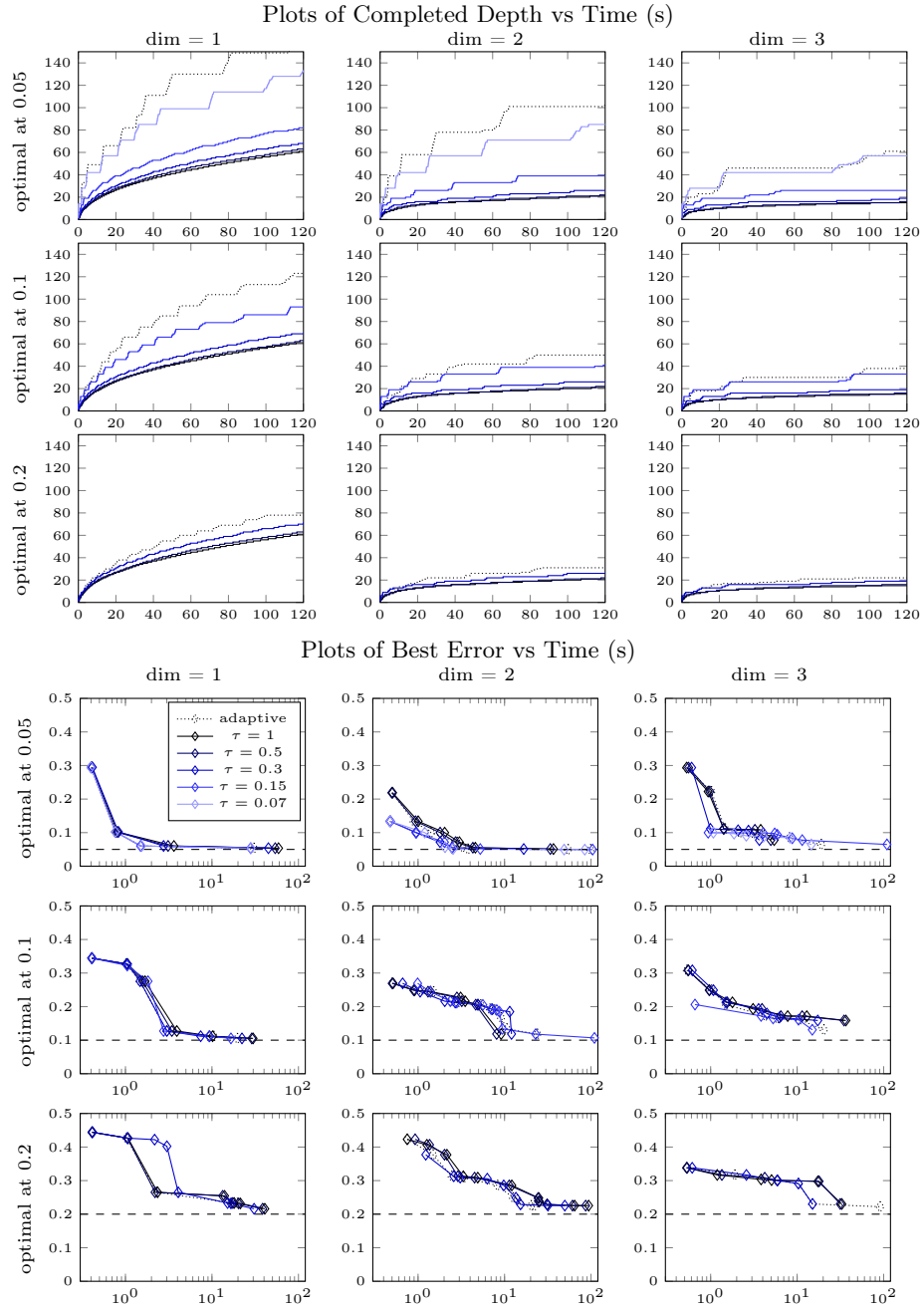
Fig. 6. Performance on synthetic hyperrectangle examples with varying parameters.
