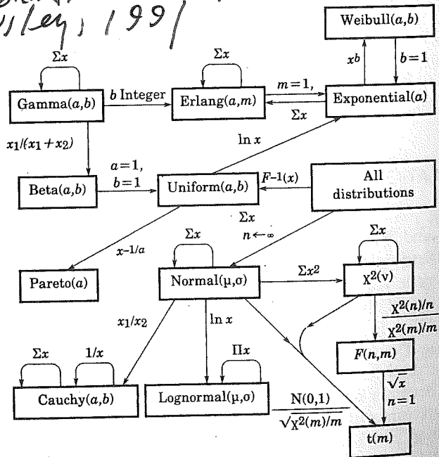
FIGURE 29.2 Relationships among continuous distributions.
