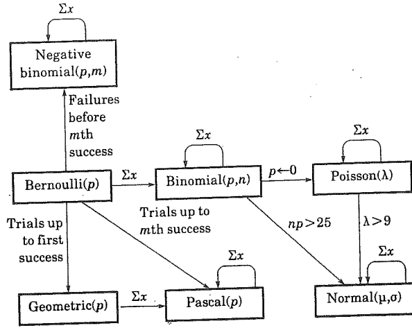
FIGURE 29.1 Relationships among discrete distributions.
