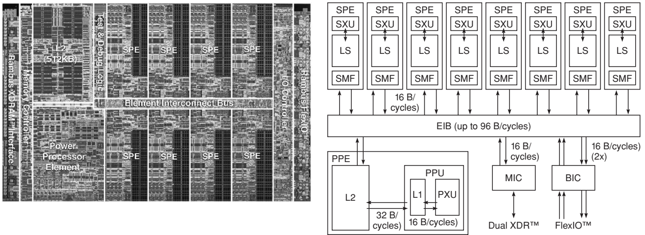
Figure E.25 Cell Broadband Engine (a) die photo and (b) high-level block diagram illustrating the function of the EIB. © IBM Corporation, 2005. All rights reserved.
