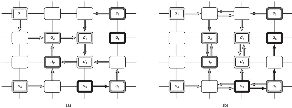
Figure E.17 A mesh network with packets routing from sources, s_i , to destinations, d_i . (a) Deadlock forms from packets destined to d_1 through d_4 blocking on others in the same set that fully occupy their requested buffer resources one hop away from their destinations. This deadlock cycle causes other packets needing those resources also to block, like packets from s_5 destined to d_5 that have reached node s_3 . (b) Deadlock is avoided using dimension-order routing. In this case, packets exhaust their routes in the X dimension before turning into the Y dimension in order to complete their routing.
