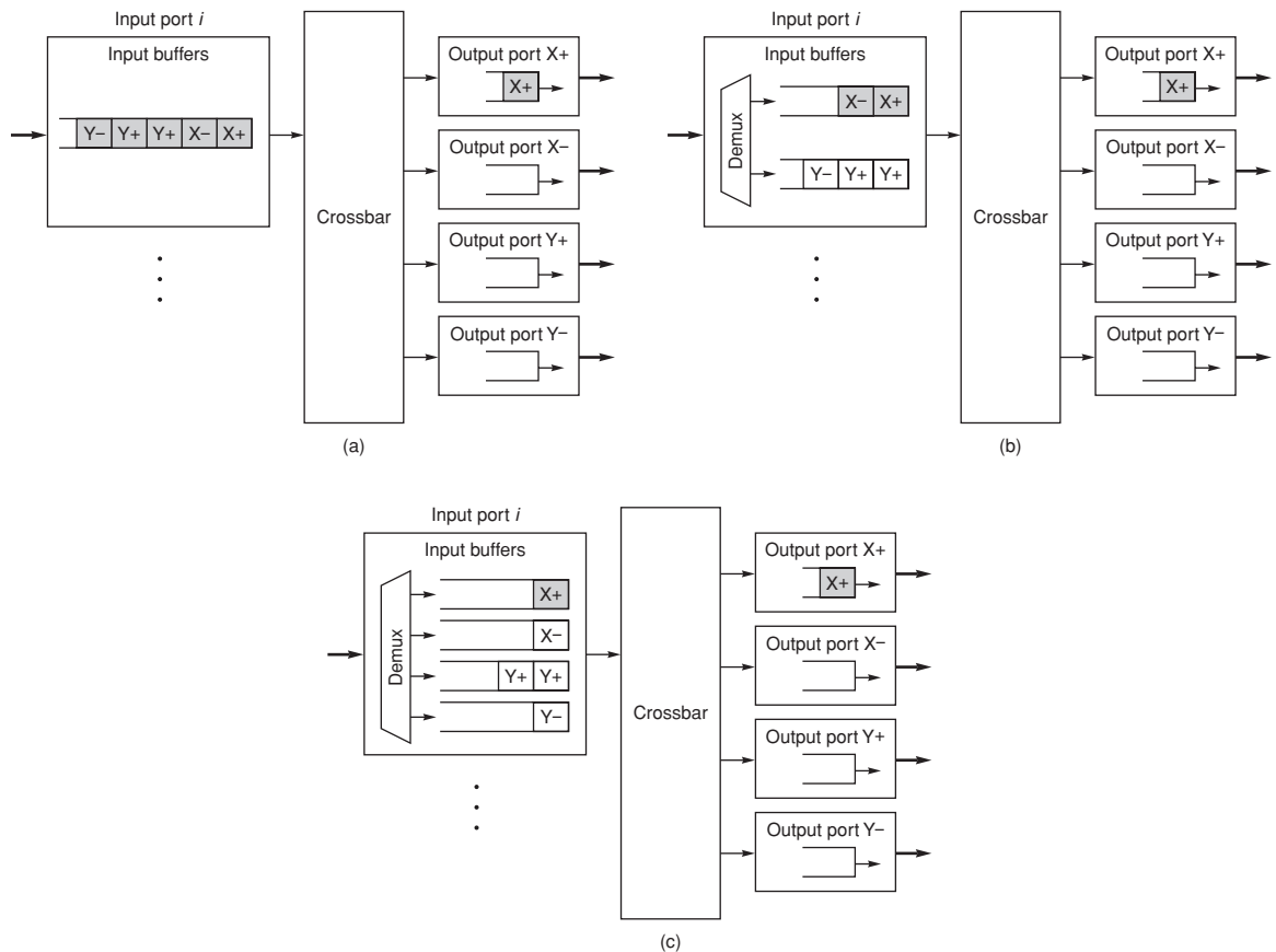
Figure E.22 (a) Head-of-line blocking in an input buffer, (b) the use of two virtual channels to reduce HOL blocking, and (c) the use of virtual output queuing to eliminate HOL blocking with a switch. The shaded input buffer is the one to which the crossbar is currently allocated. This assumes each input port has only one access port to the switch's internal crossbar.
