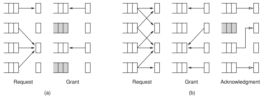
Figure E.18 Two arbitration techniques. (a) Two-phased arbitration in which two of the four input ports are granted requested output ports. (b) Three-phased arbitration in which three of the four input ports are successful in gaining the requested output ports, resulting in higher switch utilization.
