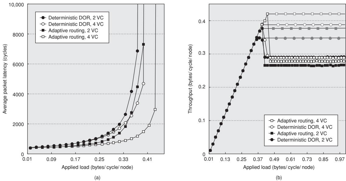
Figure E.19 Deterministic routing is compared against adaptive routing, both with either two or four virtual channels, assuming uniformly distributed traffic on a 4K node 3D torus network with virtual cut-through switching and bubble flow control to avoid deadlock. (a) Average latency is plotted versus applied load, and (b) throughput is plotted versus applied load (the upper grayish plots show peak throughput, and the lower black plots show sustained throughput). Simulation data were collected by P. Gilabert and J. Flich at the Universidad Politècnica de València, Spain (2006).
