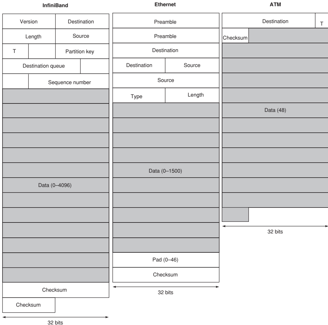
Figure E.27 Packet format for InfiniBand, Ethernet, and ATM. ATM calls their messages “cells” instead of packets, so the proper name is ATM cell format. The width of each drawing is 32 bits. All three formats have destination addressing fields, encoded differently for each situation. All three also have a checksum field to catch transmission errors, although the ATM checksum field is calculated only over the header; ATM relies on higher-level protocols to catch errors in the data. Both InfiniBand and Ethernet have a length field, since the packets hold a variable amount of data, with the former counted in 32-bit words and the latter in bytes. InfiniBand and ATM headers have a type field (T) that gives the type of packet. The remaining Ethernet fields are a preamble to allow the receiver to recover the clock from the self-clocking code used on the Ethernet, the source address, and a pad field to make sure the smallest packet is 64 bytes (including the header). InfiniBand includes a version field for protocol version, a sequence number to allow in-order delivery, a field to select the destination queue, and a partition key field. Infiniband has many more small fields not shown and many other packet formats; above is a simplified view. ATM’s short, fixed packet is a good match to real-time demand of digital voice.
