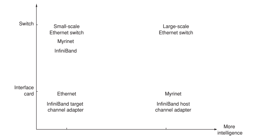
Figure E.36 Intelligence in a network: switch versus network interface card. Note that Ethernet switches come in two styles, depending on the size of the network, and that InfiniBand network interfaces come in two styles, depending on whether they are attached to a computer or to a storage device. Myrinet is a proprietary system area network.
