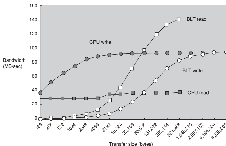
Figure E.37 Bandwidth versus transfer size for simple memory access instructions versus a block transfer device on the Cray Research T3D. (From Arpaci et al. [1995].)
