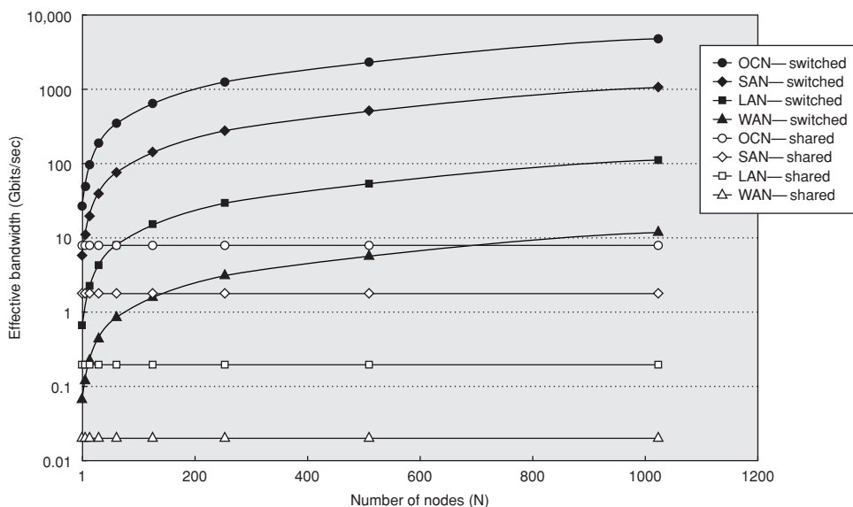
Figure E.10 Effective bandwidth versus number of interconnected nodes plotted in semi-log form for the four network domains. The disparity in effective bandwidth between shared- and switched-media networks for all interconnect domains widens significantly as the number of nodes in the network increases. Only the switched on-chip network is able to achieve an effective bandwidth equal to the aggregate bandwidth for the parameters given in this example.
