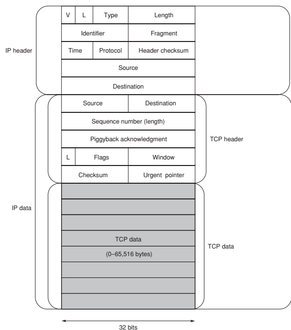
Figure E.35 The headers for IP and TCP. This drawing is 32 bits wide. The standard headers for both are 20 bytes, but both allow the headers to optionally lengthen for rarely transmitted information. Both headers have a length of header field (L) to accommodate the optional fields, as well as source and destination fields. The length field of the whole datagram is in a separate length field in IP, while TCP combines the length of the datagram with the sequence number of the datagram by giving the sequence number in bytes. TCP uses the checksum field to be sure that the datagram is not corrupted, and the sequence number field to be sure the datagrams are assembled into the proper order when they arrive. IP provides checksum error detection only for the header, since TCP has protected the rest of the packet. One optimization is that TCP can send a sequence of datagrams before waiting for permission to send more. The number of datagrams that can be sent without waiting for approval is called the window , and the window field tells how many bytes may be sent beyond the byte being acknowledged by this datagram. TCP will adjust the size of the window depending on the success of the IP layer in sending datagrams; the more reliable and faster it is, the larger TCP makes the window. Since the window slides forward as the data arrive and are acknowledged, this technique is called a sliding window protocol . The piggyback acknowledgment field of TCP is another optimization. Since some applications send data back and forth over the same connection, it seems wasteful to send a datagram containing only an acknowledgment. This piggyback field allows a datagram carrying data to also carry the acknowledgment for a previous transmission, “piggybacking” on top of a data transmission. The urgent pointer field of TCP gives the address within the datagram of an important byte, such as a break character. This pointer allows the application software to skip over data so that the user doesn’t have to wait for all prior data to be processed before seeing a character that tells the software to stop. The identifier field and fragment field of IP allow intermediary machines to break the original datagram into many smaller datagrams. A unique identifier is associated with the original datagram and placed in every fragment, with the fragment field saying which piece is which. The time-to-live field allows a datagram to be killed off after going through a maximum number of intermediate switches no matter where it is in the network. Knowing the maximum number of hops that it will take for a datagram to arrive—if it ever arrives—simplifies the protocol software. The protocol field identifies which possible upper layer protocol sent the IP datagram; in our case, it is TCP. The V (for version) and type fields allow different versions of the IP protocol software for the network. Explicit version numbering is included so that software can be upgraded gracefully machine by machine, without shutting down the entire network. In 2006, version six of the Internet protocol (IPv6) was widely used.
