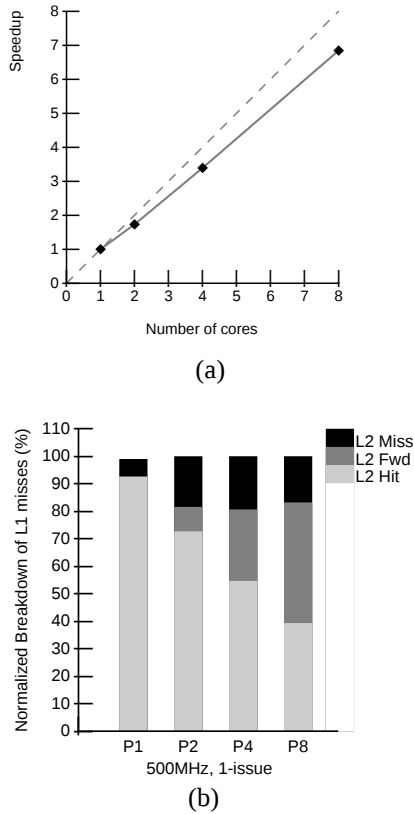
Figure 6. Piranha’s (a) speedup and (b) L1 miss breakdown for OLTP.
