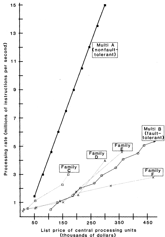
Fig. 3. Performance is plotted against price for two multis (A and B) and several conventional computer families. C, D, and E are families of minicomputers; F is a family of mainframe computers. The cost-effectiveness of a multi is achieved by its use of the same components to cover a range of functions as opposed to the individual design, semiconductor technology, and packaging required for each member of a traditional computer family.
