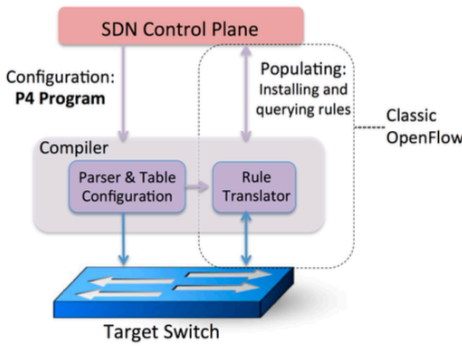
Figure 1: P4 is a language to configure switches.
