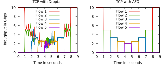
Figure 14: Convergence test
