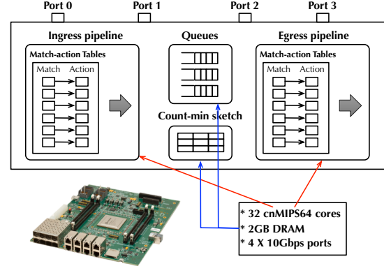
Figure 6: High-level architecture of the AFQ switch prototype.
