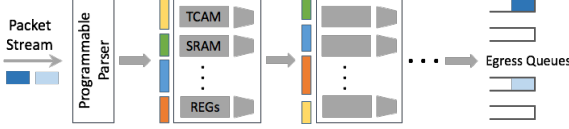
Figure 2: The architecture of a reconfigurable switch. Packets are processed by a pipeline of match+action stages with local state.
