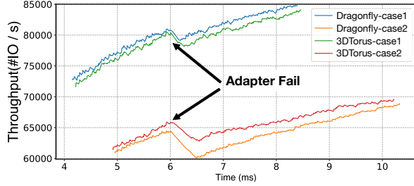
Figure 16: Perf. under an adapter failure in a switchless SAN. the end-to-end storage control.
