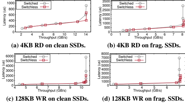
Figure 11: Latency versus throughput for 4KB random read and 128KB sequential write on clean and fragmented SSDs.
