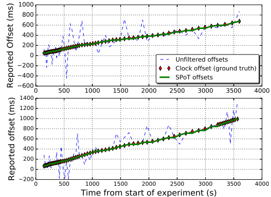
Figure 2: Offsets of IoT devices 1 (top) and 2 (bottom) reported by SPoT from the first hour of the experiment with high noise level.
