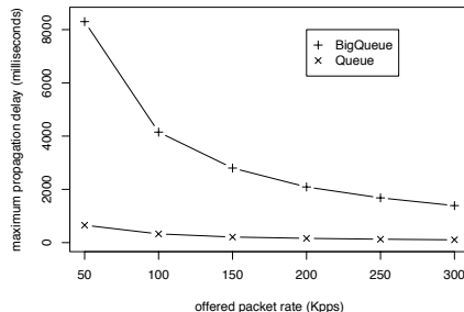
Figure 4. Maximum propagation delays possible with the standard Click Queue element compared with the enhanced BigQueue element.
