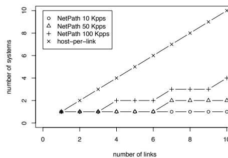
(b) Number of host systems required for NetPath under different maximum link loads. A one-host-per-link reference line is also shown as this is the approach used in some network testbeds today.
