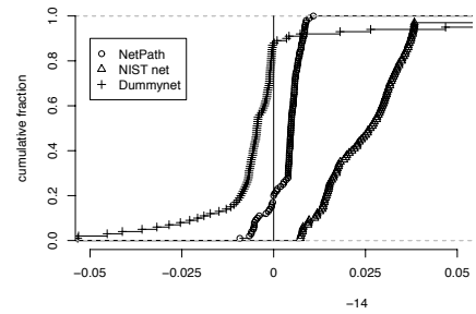
Figure 10. Distribution of response times (time between initial SYN and first data response packet) for web-like TCP traffic using NetPath, NIST net, and Dummysnet. Response times are all relative to the Adtech SX-14.
