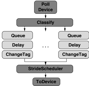
Figure 1. Click elements used in basic and multiple link emulation. Lighter elements were modified and extended for NetPath.
