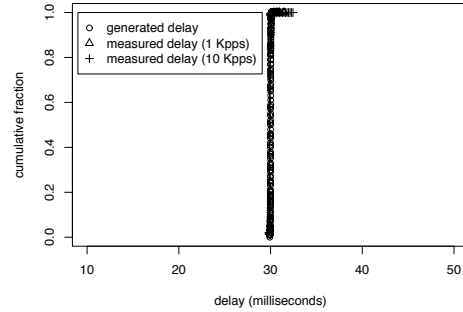
(b) Generated delay of mean 30 millisecond and standard deviation 30 microsecond.
