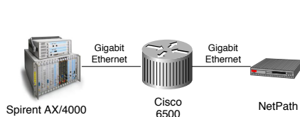
(a) In our basic setup, constant rate UDP streams produced by the AX/4000 were redirected to NetPath via a Cisco 6500 switch. After NetPath processing, packets returned to the AX/4000, where propagation delays and loss rates were measured.
