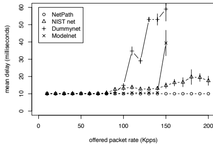
Figure 8. Delay precision of NetPath, NIST net, Dummysnet and Modelnet respectively for a configured delay of 10 millisecond. Lines above and below each curve represent one standard deviation away from mean.
