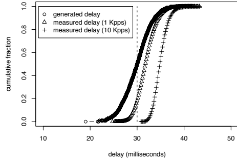
(a) Generated delay of mean 30 millisecond and standard deviation 3 millisecond.
