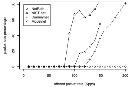
Figure 9. Comparison of packet loss characteristics of NetPath versus other popular software-based emulators under different offered packet rates.
