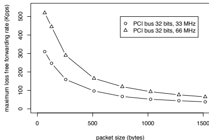
Figure 3. NetPath’s throughput as a function of packet size for two different host PCI bus configurations.
