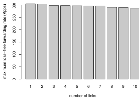
(a) Maximum loss-free forwarding rate of one NetPath host with multiple links. Offered load is spread evenly across all links.
