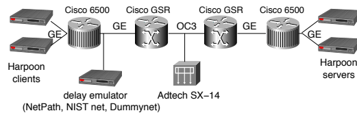
(b) An extended setup was used for evaluating application traffic performance under different path emulation systems. We generated self-similar web-like TCP flows using the Harpoon traffic generator across a dumbbell-like topology.
