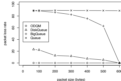
Figure 5. Packet loss rates for four different queue implementations. Offered loads are fixed at 100 Mb/s with varying packet sizes. NetPath is configured to limit link capacity to 10 Mb/s.
