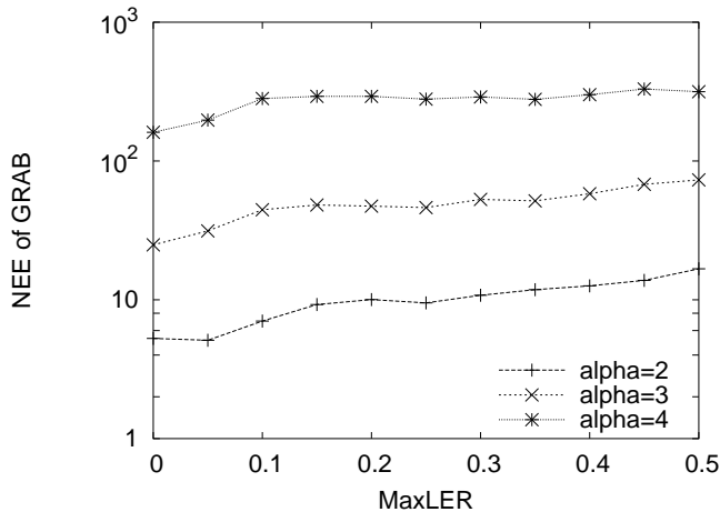
Figure 6: Normalized energy efficiency of GRAB.
