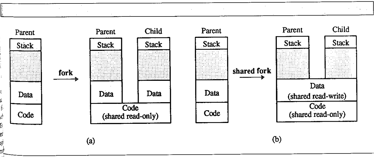
Figure 2. The Unix fork operation (a) creates a new process that shares code with its parent while using private copies of the data and stack segments. Sprite provides both the traditional fork and a shared fork (b) in which the child shares its parent's data as well as code.
