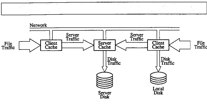
Figure 6. Caches in the Sprite file system. When a process makes a file access, it is presented first to the cache of the process' workstation (file traffic). If not satisfied there, the request is passed either to a local disk, if the file is stored locally (disk traffic), or to the server where the file is stored (server traffic). Servers also maintain caches to reduce their disk traffic.
