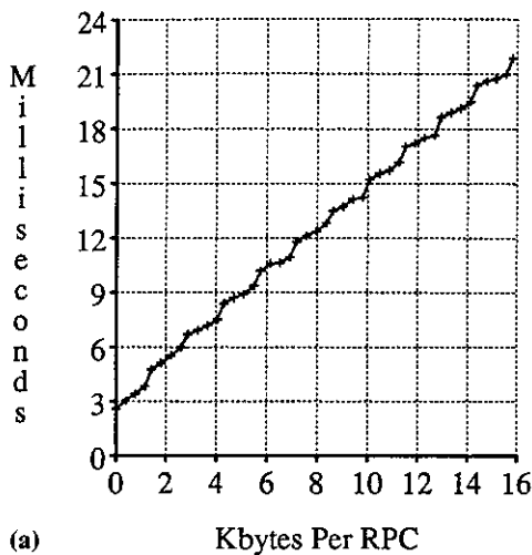
Figure 4. Measured performance of Sprite's remote procedure call mechanism between Sun-3/75 workstations. The test consisted of one kernel invoking a remote procedure in another kernel, passing to it the contents of a variable-size array as an argument. The called procedure returned immediately. Part (a) shows the round-trip time for an individual RPC as a function of the amount of data passed to the remote procedure; (b) shows the throughput when repeated RPCs are made. Larger transfers, which use fragments on 1500-byte boundaries, are most efficient. The jumps in the curves occur at the points where additional packets become necessary.
