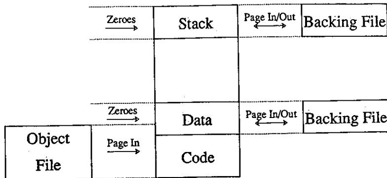
Figure 9. Sprite's paging structure. The code is paged in on-demand from the process' object file; since the code is read-only, it need not be written to backing storage and can be reloaded from the object file when needed. An ordinary file is used to back each data and stack segment. Initialized portions of the data segment are read in from the object file on first reference, then written to the backing file during page replacement and reused from there. For the stack segment and the uninitialized portions of the data segment, pages are filled with zeroes on first reference, then paged to and from the backing files.
