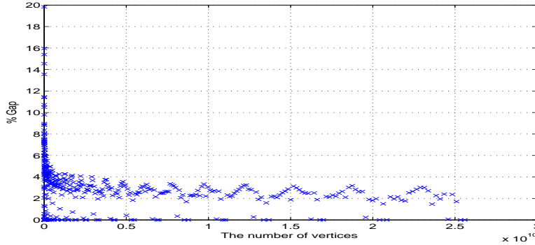
FIG. 5.3. Gap% versus the number of vertices ( M^4 ) for MSA([M]^4, M^2) ( 1 \leq M \leq 400 )
