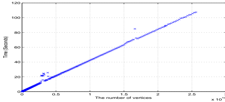
FIG. 5.4. Execution time versus the number of vertices ( M^3 ) for MSA([M]^4, M^2) ( 1 \leq M \leq 400 )
