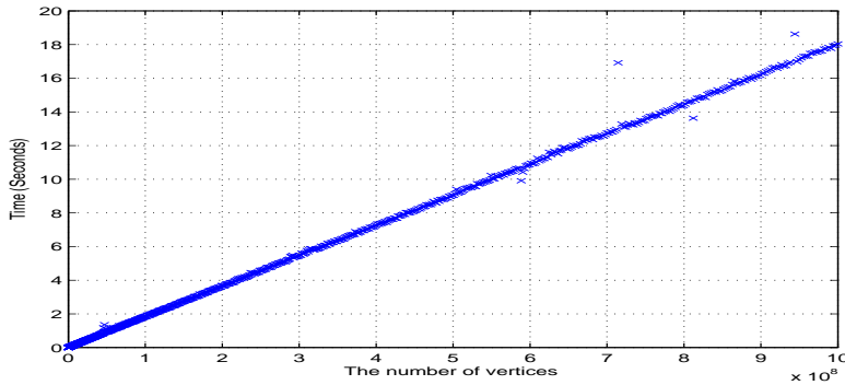
FIG. 5.2. Execution time versus the number of vertices ( M^3 ) for MSA([M]^3, M) ( 1 \leq M \leq 1000 )
