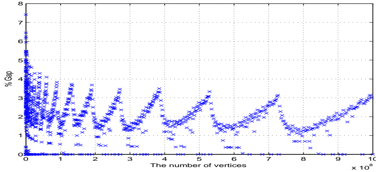
FIG. 5.1. Gap\% versus the number of vertices ( M^3 ) for MSA([M]^3, M) ( 1 \leq M \leq 1000 )
