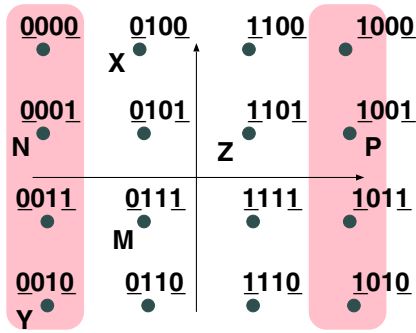
Figure 4: 16-QAM with Gray code constellation map. MSBs and LSBs are underlined.
