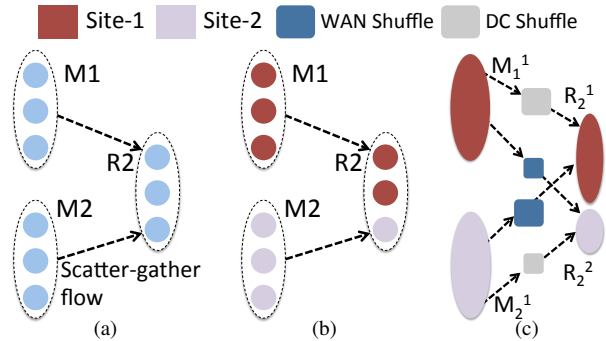
Figure 6: (a) shows a simple MR job with 3 tasks in each stage. (b) shows the same job with placement information (color-coded) for all the tasks. (c) shows the corresponding augmented DAG with tasks in the same stage and location coalesced to one. M_* and R_* are sub-stages in the augmented DAG. Shuffle tasks representing network transfer between tasks at different locations are shown explicitly.
