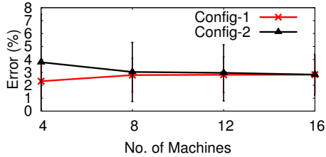
Figure 12: The errors from two cluster scenarios with different number of nodes. Config-1: strong-scaling to fix the total number of estimators as 2M \times 128 ; Config-2: weak-scaling to fix the number of estimators per executor as 2M .
