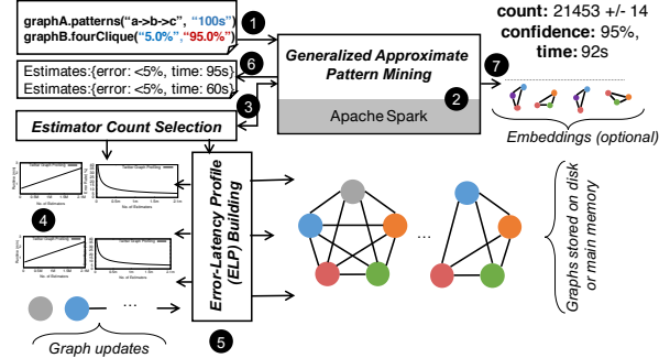
Figure 3: ASAP architecture
