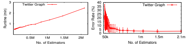
Figure 7: The actual relations between number of estimators and run-time or error rate.
