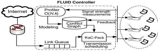
Figure 4: Flow of operations in FLUID. Periodic signal strength measurements are used to update the modeled conflict graph (§4). Packets arrive from the network gateway and are enqueued at a central controller. The controller releases these packets based on the transmission schedules derived by a packing algorithm (§5). APs receive the packets and transmit them according to the controller’s prescribed flexible channel assignment, and subsequently notify the controller of all failures. The controller uses this feedback for scheduling retransmissions and refining the conflict graph.
