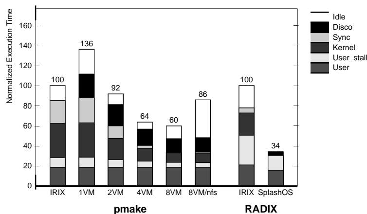
Fig. 8. Workload scalability under Disco
