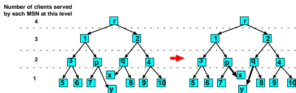
Fig. 8. Example where the five local operations cannot lead to optimality in the min avg-latency problem. All MSNs have maximum out-degree bound of two. r is the root. Arrow lengths indicate the distance between MSNs.
