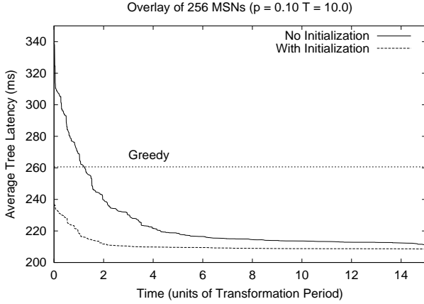
Fig. 14. Effect of the initialization phase (256 MSNs).
