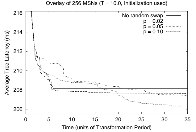
Fig. 15. Varying the probability of performing the random-swap operation for the different MSNs (256 MSNs).
