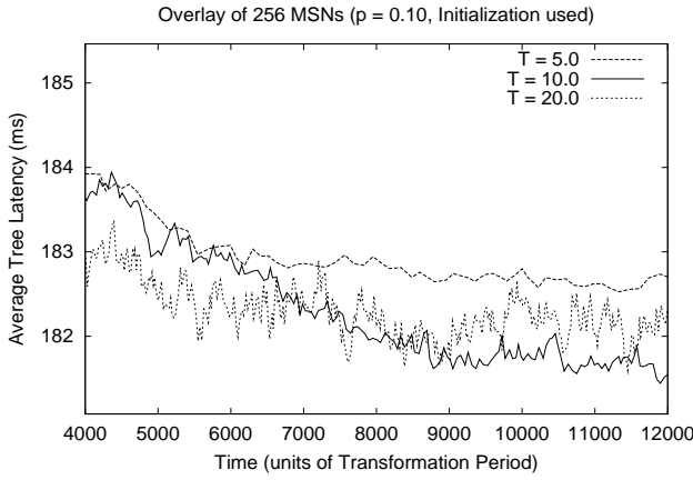
Fig. 16. Varying the temperature parameter for simulated annealing (256 MSNs).
