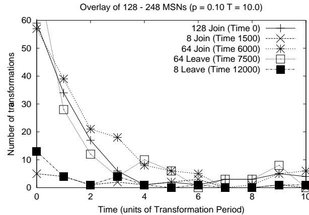
Fig. 18. Distribution of number of transformations in the first 10 transformation periods after a set of changes happen in the join leave experiment with 248 MSNs.
