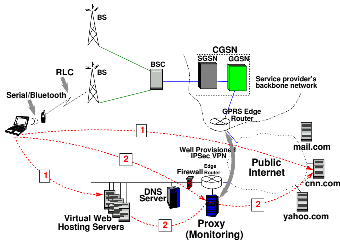
Fig. 1. WWAN Architecture and Testbed. In these experiments, we placed the proxy in our laboratory and then use a well provisioned IPsec VPN to ‘back haul’ GPRS traffic to it directly from the cellular provider’s network. In the proxy-based experiments, the mobile client connects to the web servers through this proxy (Label 2 in Figure 1).
