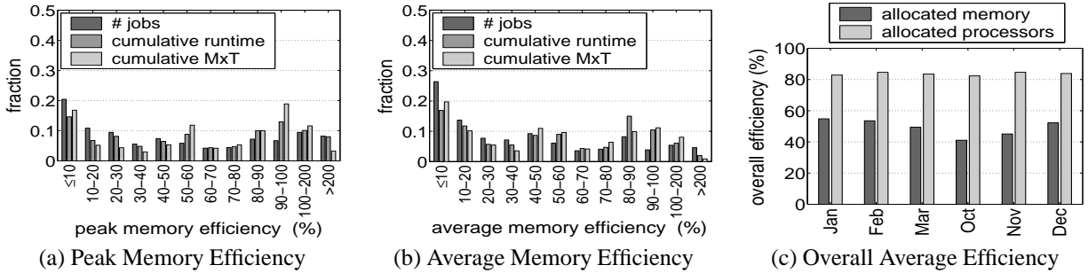
Figure 16. Memory Efficiency
