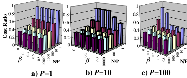
Figure 8: Cost Ratio of BWSkim(2) to BWSkim(1.2) (unconstrained proxy servers, one file)
