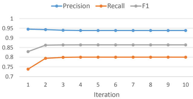
Fig. 4. Precision, recall, and F1 score over 400 random sample sentences
