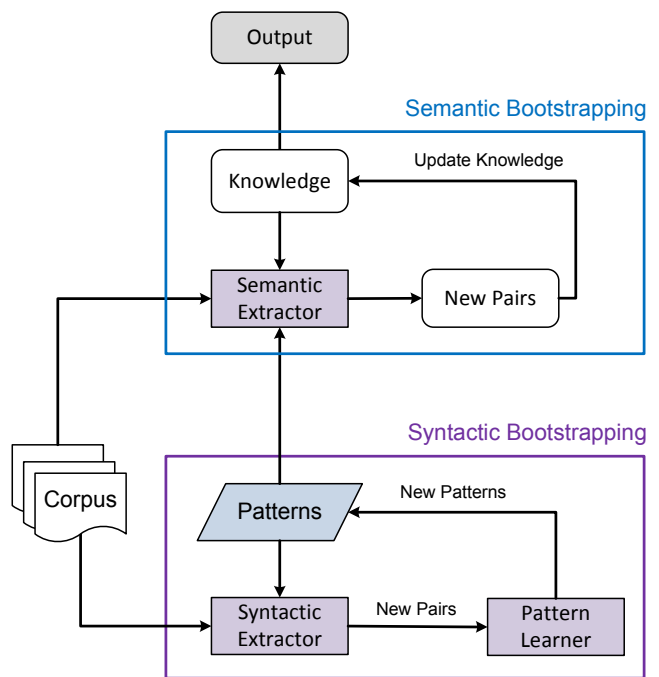
Fig. 5. Combine syntactic and semantic bootstrapping
