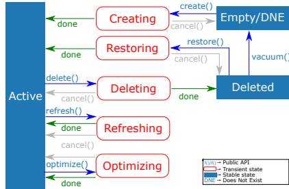
Figure 6: Index State Machine
