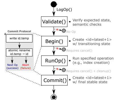
Figure 7: Log Operation
